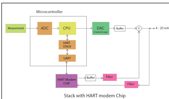
Example Block Diagram with External HART Modem Chip
